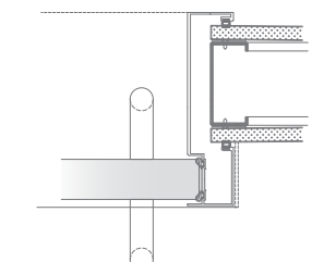
4 JAMB @ PULL SIDE Typical
