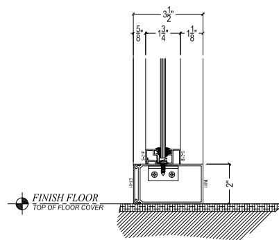
A STANDARD SILL OPTION USING IM-01 At SideLite
