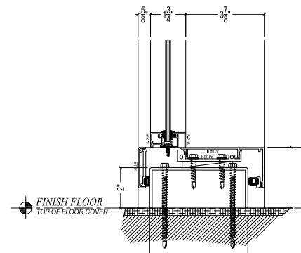
B FULL DEPTH OPTION At SideLite
