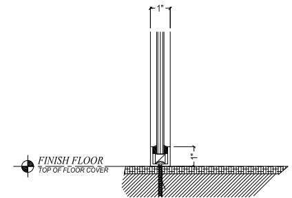
C U-CHANNEL OPTIONS At SideLite
